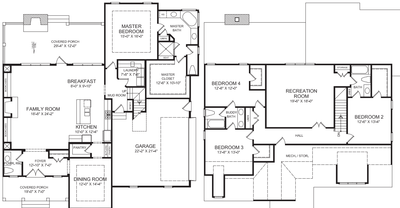
FIRST FLOOR
